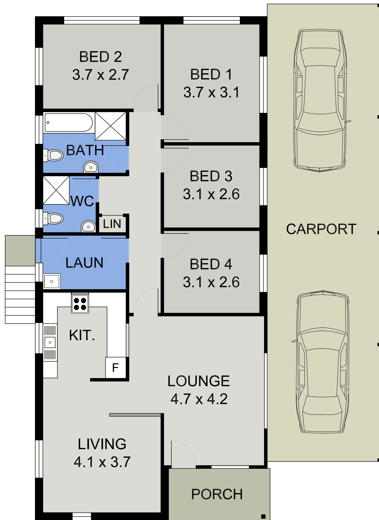
FLOOR PLAN
