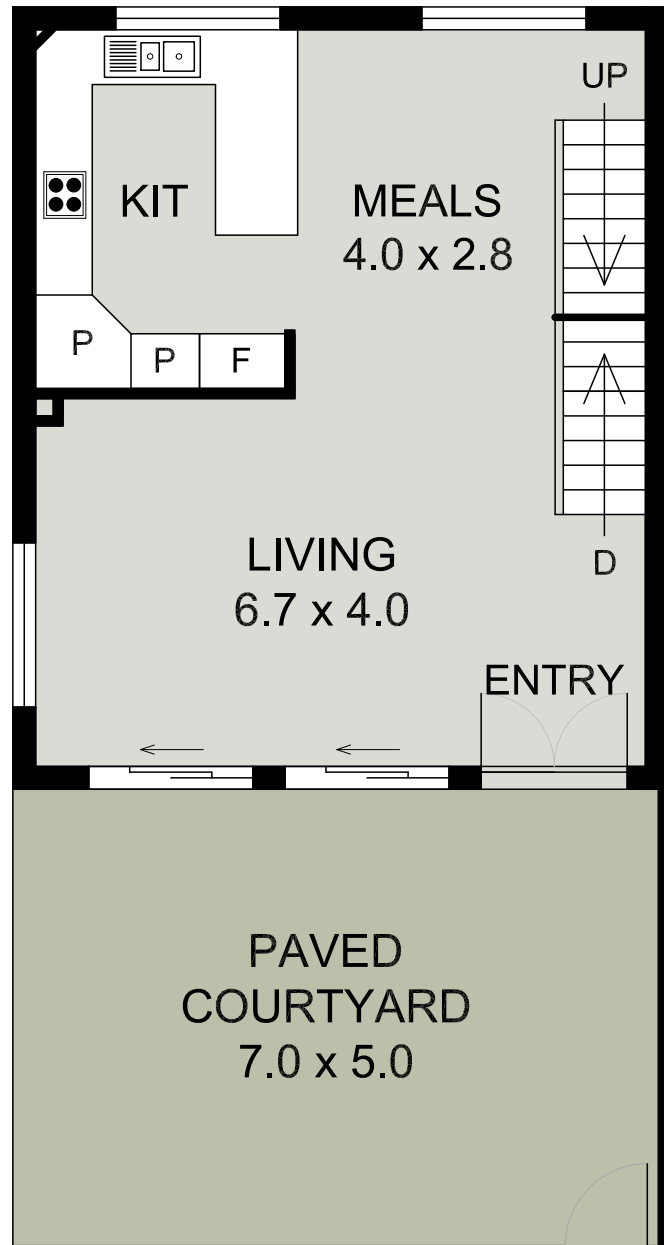
MIDDLE FLOOR PLAN
