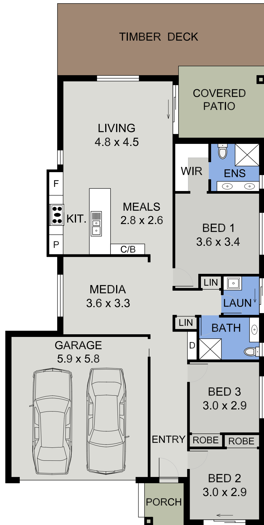
FLOOR PLAN
