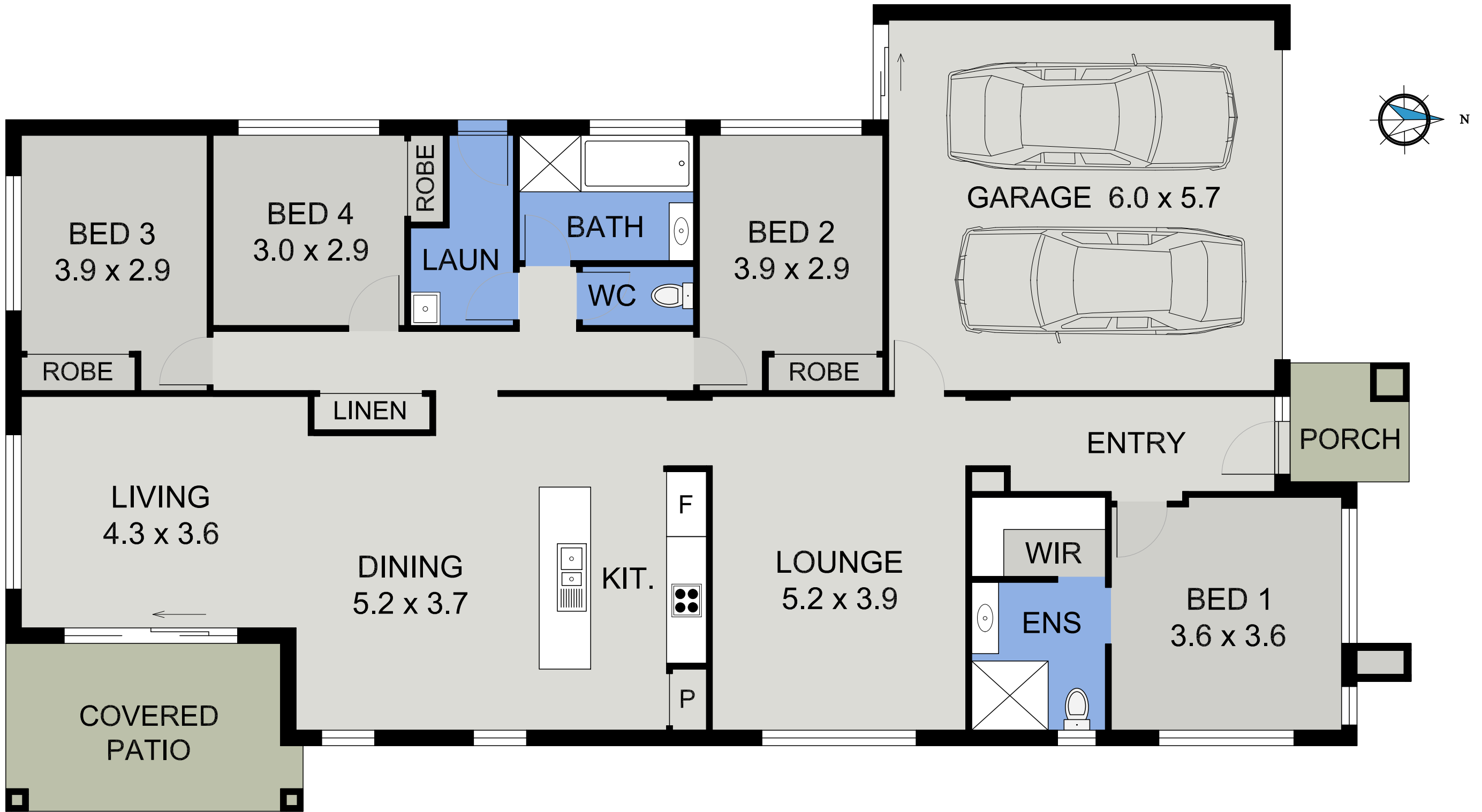
FLOOR PLAN
