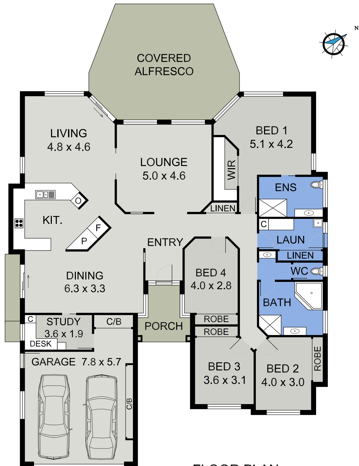
FLOOR PLAN
