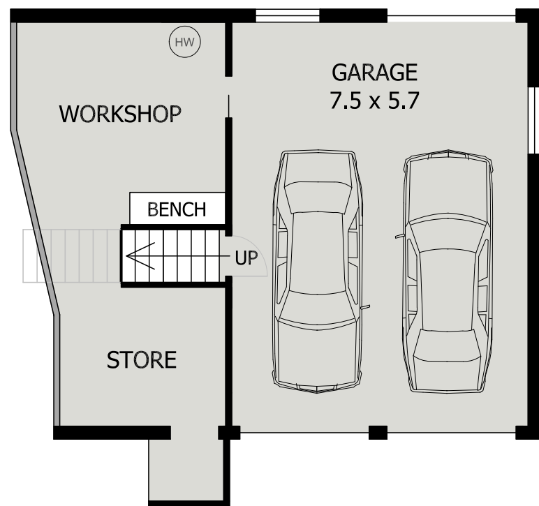
LOWER FLOOR PLAN
