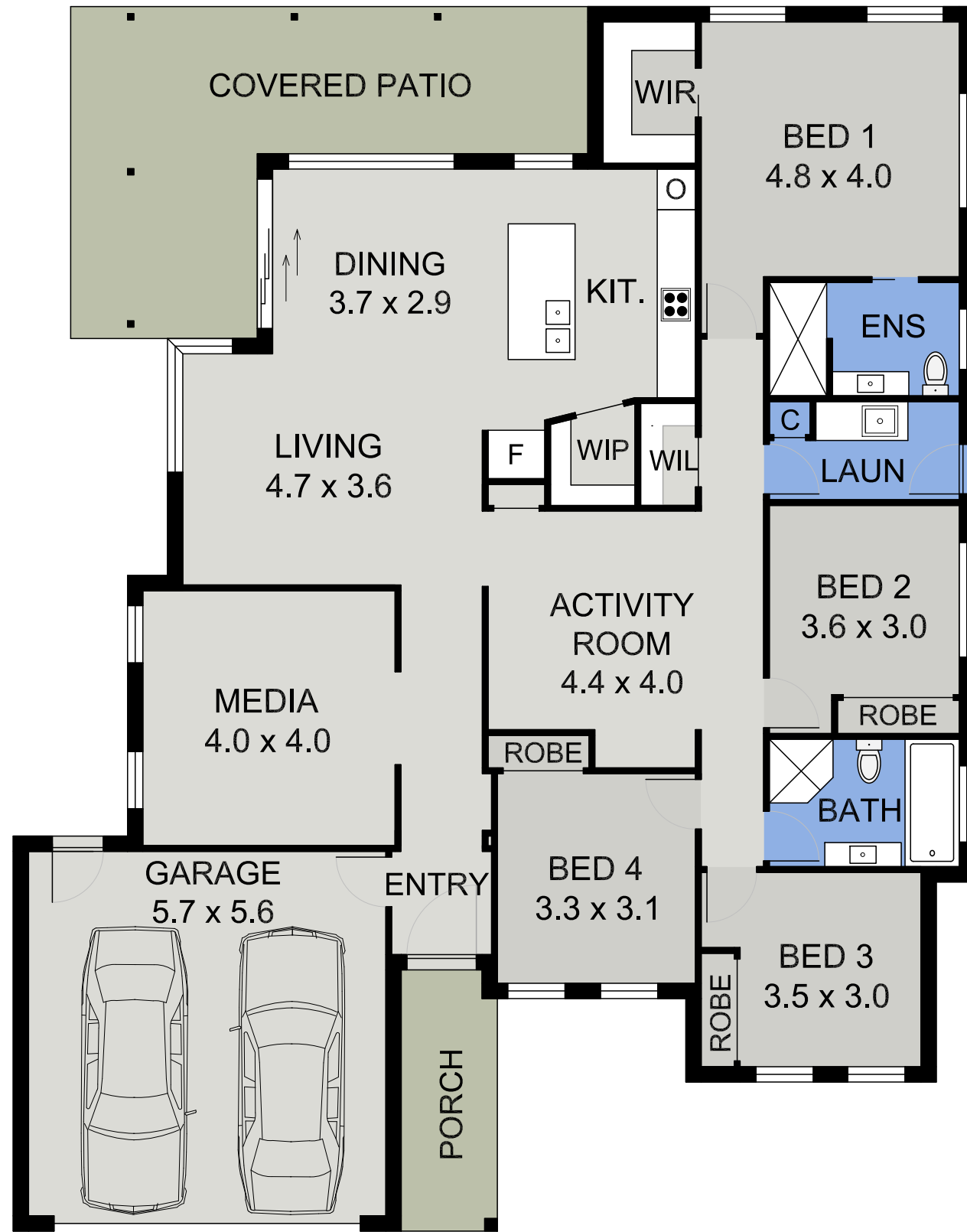
FLOOR PLAN
