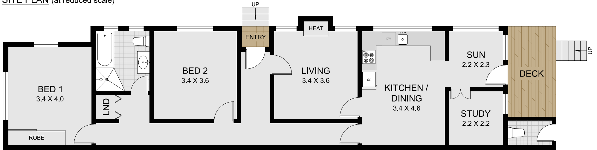
SITE PLAN (at reduced scale)
